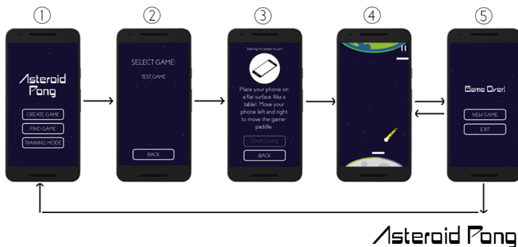
Figure 15: User flow diagram of how to connect to a created multiplayer game
