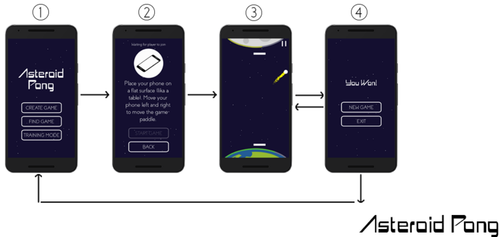
Figure 14: User flow diagram of how to create a multiplayer game
