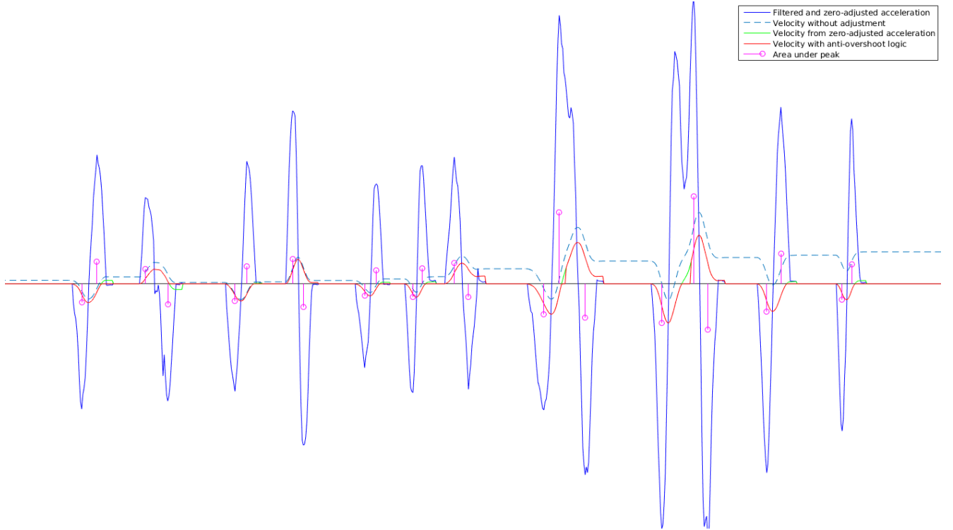
Figure 10: A visulization of actual real time data gathered from the Android application, and processed in Matlab
