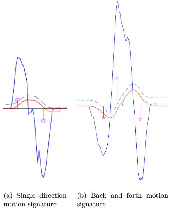
Figure 11: The two most common user motion signatures
