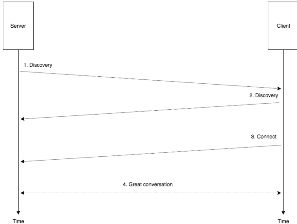
Figure 8: The wifi direct setup procedure between two devices running Asteroid Pong
