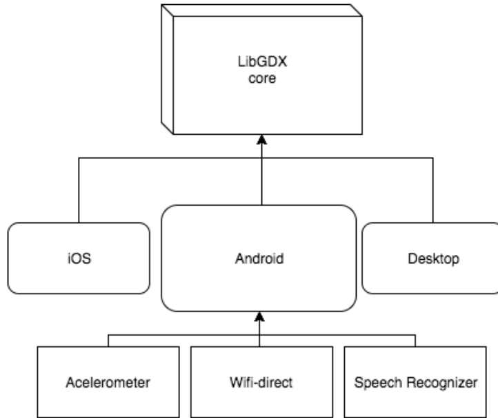
Figure 7: The different modules communicating with the LibGDX core
