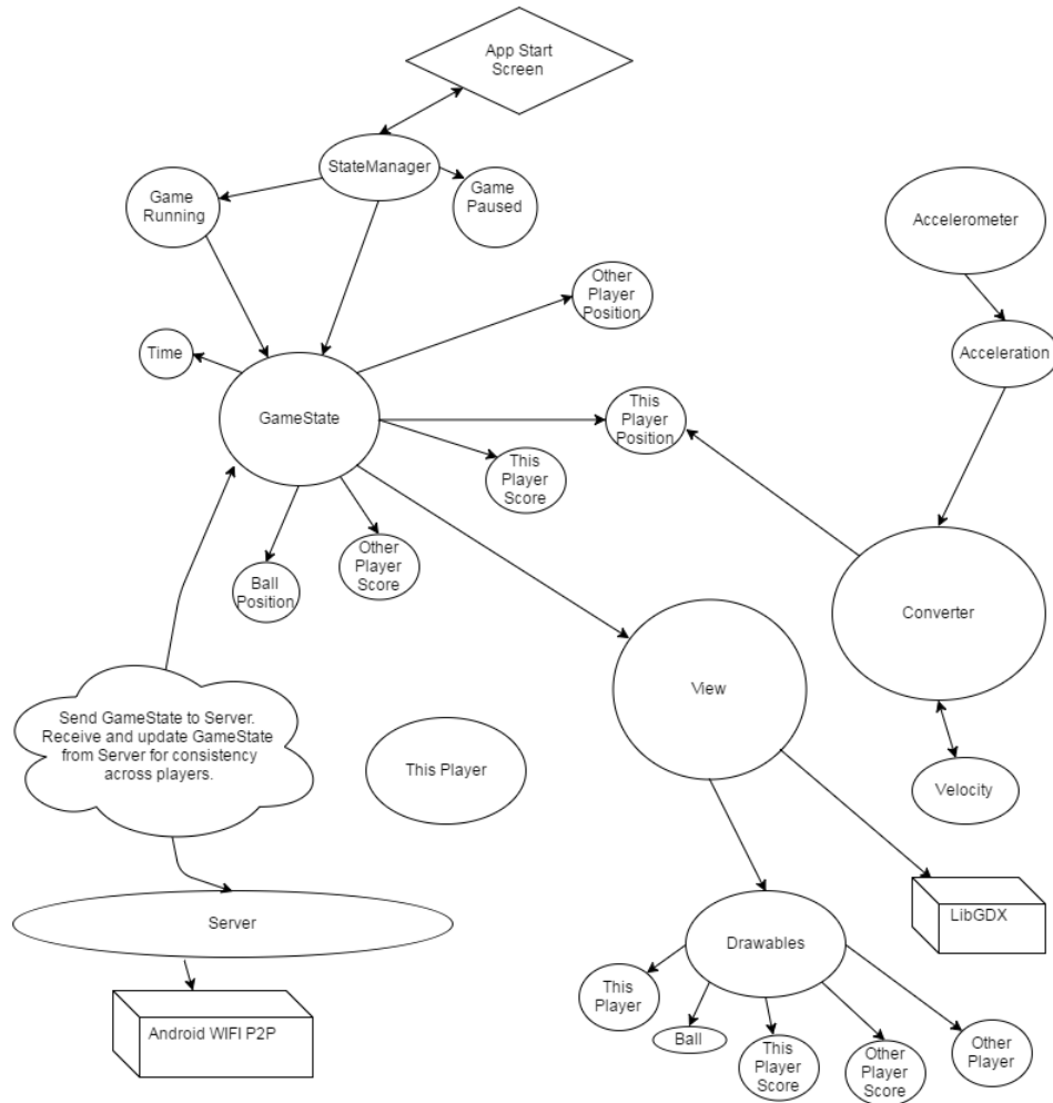
Figure 6: Structure of the project
