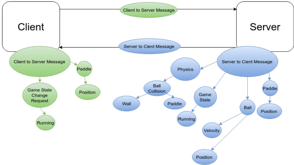
Figure 9: The network structure for messages between the client and server
